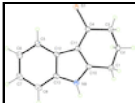
Fig. 1. View of 1 (50% probability displacement ellipsoids).
