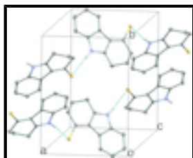
Fig. 2. The unit cell, illustrating hydrogen bonds.
